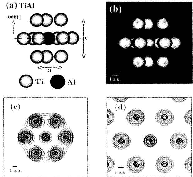
FIG. 3. Geometry and charge distribution in a very dilute TiAl alloy, represented by Ti(hcp) with a substitutional Al impurity. (a) Geometry of the Ti_{12}Al core cluster. (b) Three-dimensional (3D) representation of the total charge density surface in the Ti_{12}Al cluster, corresponding to \rho = 0.1 e^-/a.u.^3 , calculated using the DMOL all-electron cluster method. (c) Results of the same calculation, presented as a 2D contour plot in the (0001) plane, which is shown by the dashed line in (a) and contains the Al impurity. (d) Total charge density in the dilute TiAl alloy, calculated using the LMTO-ASA-Green-function method, and represented in the same manner and geometry as in (c). The ratio of two consecutive contours in (c) and (d) is \rho(n+1)/\rho(n) = 1.5 .
