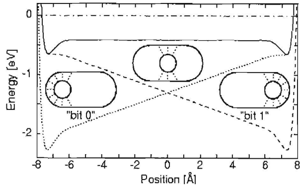
Figure 5 Potential energy of the shuttle at different locations in the capsule. The solid line is when no electric field is applied. The dashed lines are the potential energy when the two-volt potential difference is applied. [2]
