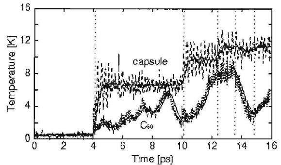
Figure 8 The heat generated by the shuttle slamming into the capsule during a write. [2]
