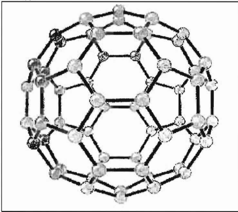
Figure 3 A buckyball
