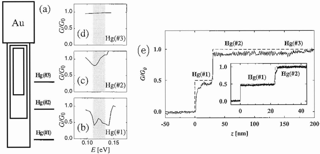
FIGURE 1. (a) Schematic geometry of a multi-wall nanotube that is being immersed into mercury up to different depths labeled Hg(#1), Hg(#2), and Hg(#3). Only the outermost tube is considered to be in contact with the gold STM tip on which it is suspended. The conductance of this system is given in (b) for the immersion depth Hg(#1), in (c) for Hg(#2), and in (d) for Hg(#3) as a function of the position of E_F . The Fermi level may shift with changing immersion depth within a narrow range indicated by the shaded region. (e) Conductance G of a multi-wall nanotube as a function of immersion depth z in mercury, given in units of the conductance quantum G_0 = 2e^2/h \approx (12.9 \text{ k}\Omega)^{-1} . Results predicted for the multi-wall nanotube, given by the dashed line, are superimposed on the experimental data of Ref. [3]. The main figure and the inset show data for two nanotube samples, which in our interpretation only differ in the length of the terminating single-wall segment. From Ref. [4], ©American Physical Society 2000.
