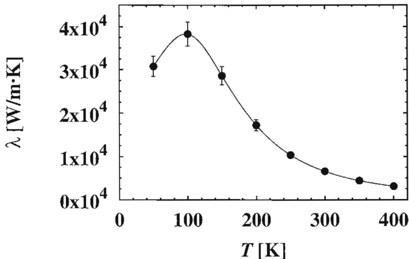
FIGURE 2. Temperature dependence of the thermal conductivity \lambda for a (10,10) carbon nanotube for temperatures below 400 K. From Ref. [18], ©American Physical Society 2000.
