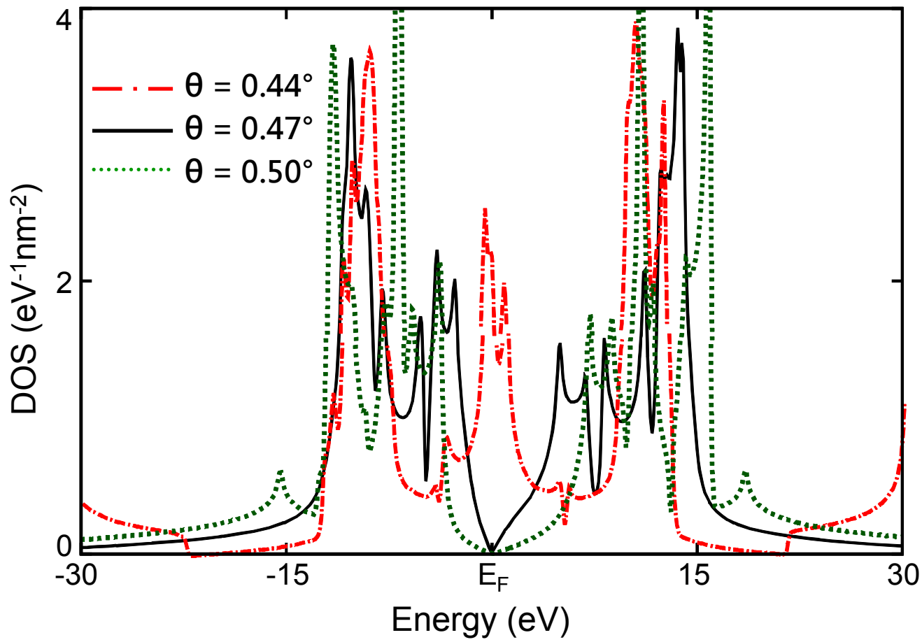
Density of states near the second magic angle \theta_{m,2} \approx 0.47^\circ
