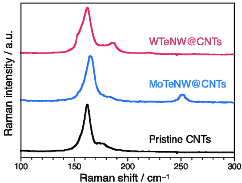
Fig. S9 Raman spectra of WTeNWs@CNT (pink), MoTeNW@CNTs (blue) and pristine CNTs (black).
